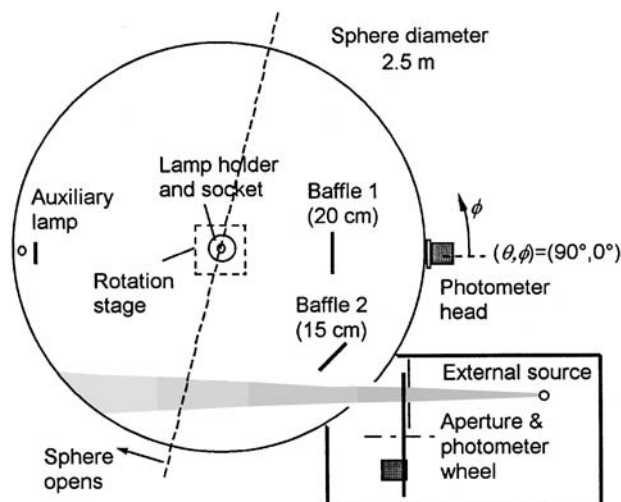
Figure 2. Arrangement of the new NIST 2.5 m integrating sphere for the detector-based luminous-flux calibration (top view).
