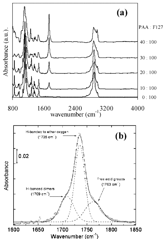
Figure 1. (a) FTIR spectra for spin-coated films of F127 and its PAA blends at various compositions. (b) Deconvoluted spectrum of C=O stretching vibrations from a 40:100 PAA:F127 blend showing the relative contributions from different interactions of COOH groups in PAA and the ether oxygen in F127.
