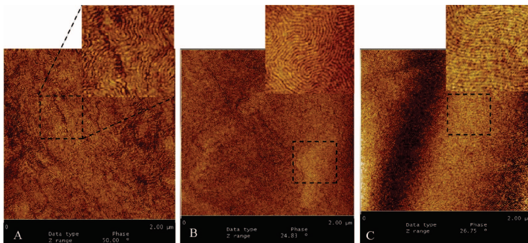
Figure 3. AFM phase images ( 2\ \mu\text{m} \times 2\ \mu\text{m} ) for spin-coated films of (A) neat F127 and its PAA blends at (B) 16.67% and (C) 28.5% by mass. Insets show magnified regions of 0.5 \times 0.5\ \mu\text{m}^2 from highlighted areas for clarity.
