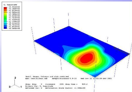
FE Analysis and Non-Linear Buckling Analysis (Rev. 2000)
