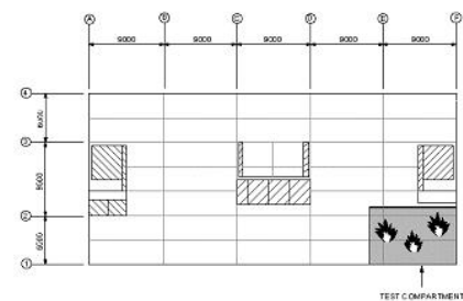
TEST 3 : CORNER COMPARTMENT TEST
