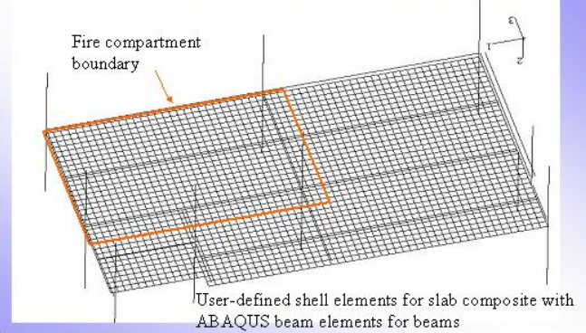
FE Analysis and Non-Linear Buckling Analysis (Rev. 2000)
