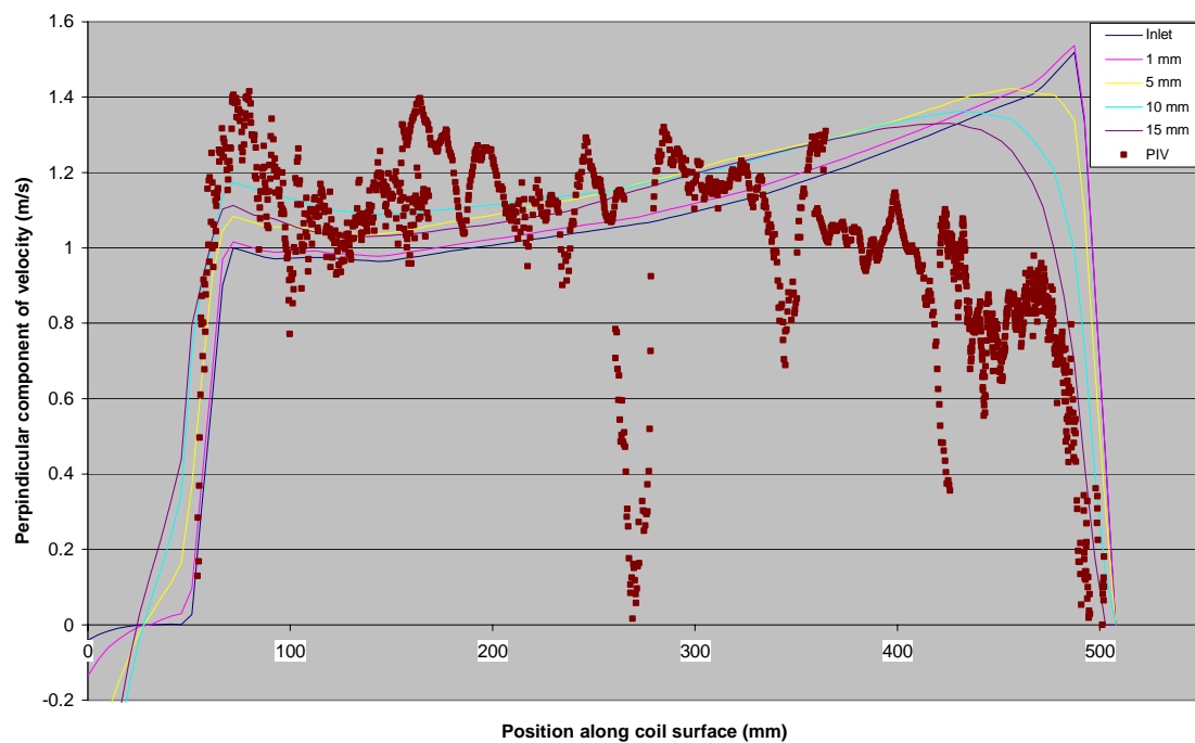
Figure 4.15 PIV and CFD data for inlet to lower slab at 1200 CFM wet coil, Test 3b
