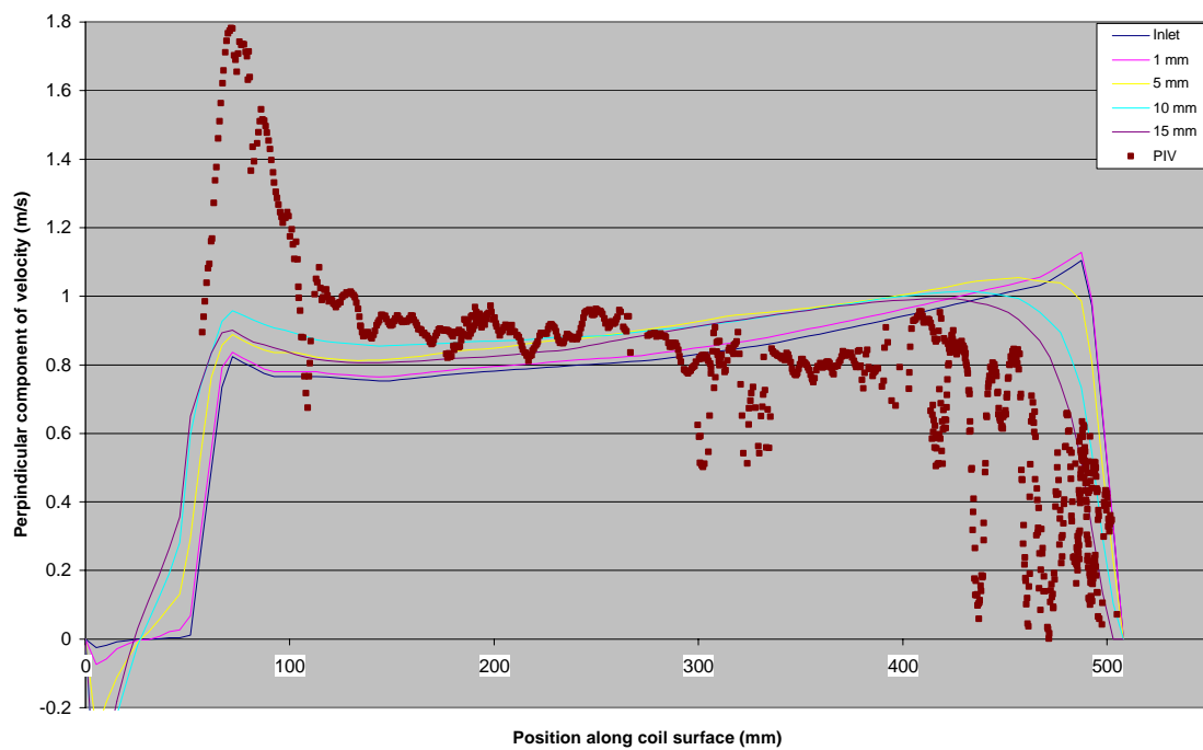
Figure 4.18 PIV and CFD data for inlet to lower slab at 900 CFM wet coil, Test 4b
