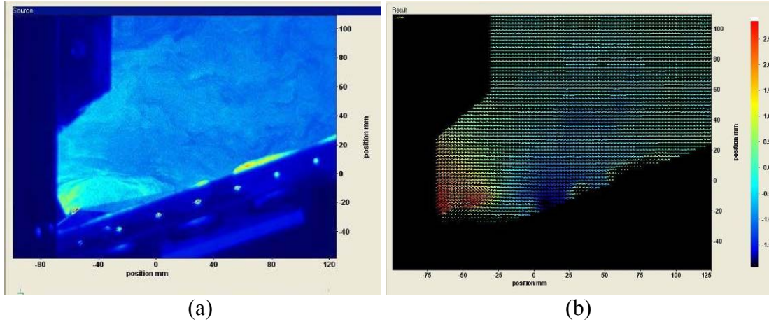
Figure 2.11 Air flow approaching bottom slab of an A-shaped coil
