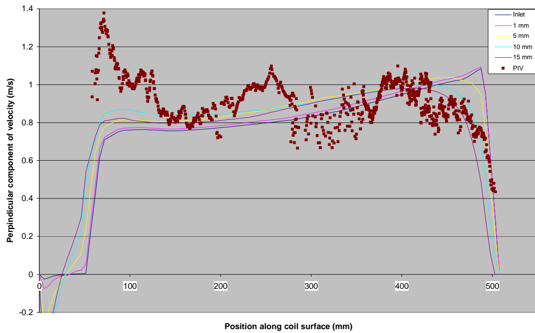
Figure 4.12 PIV and CFD data for inlet to lower slab at 900 CFM dry coil, Test 2b
