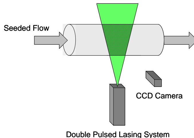
Figure 2.6 Schematic of 2-dimensional PIV setup
