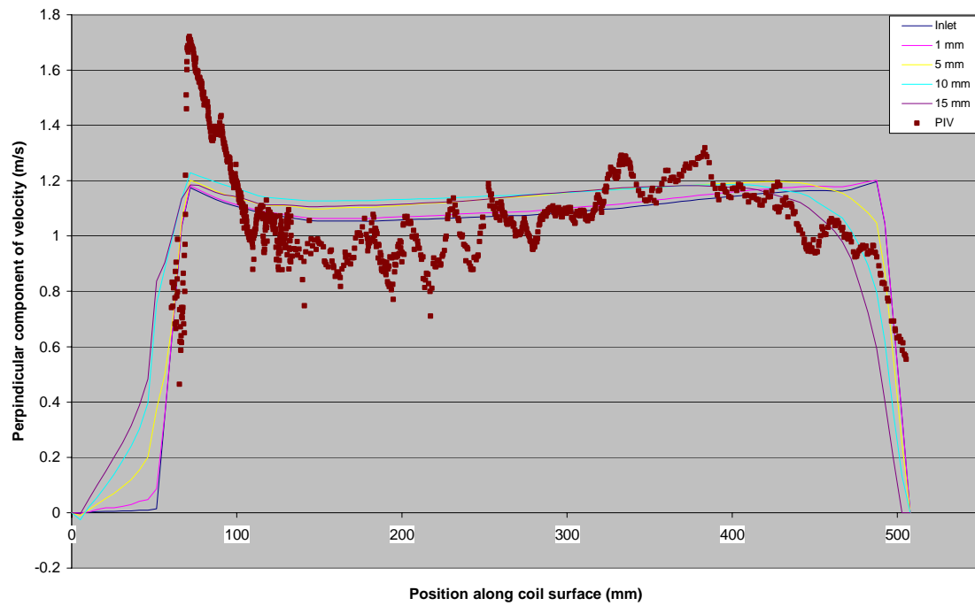
Figure 4.11 PIV and CFD data for inlet to upper slab at 900 CFM dry coil, Test 2a
