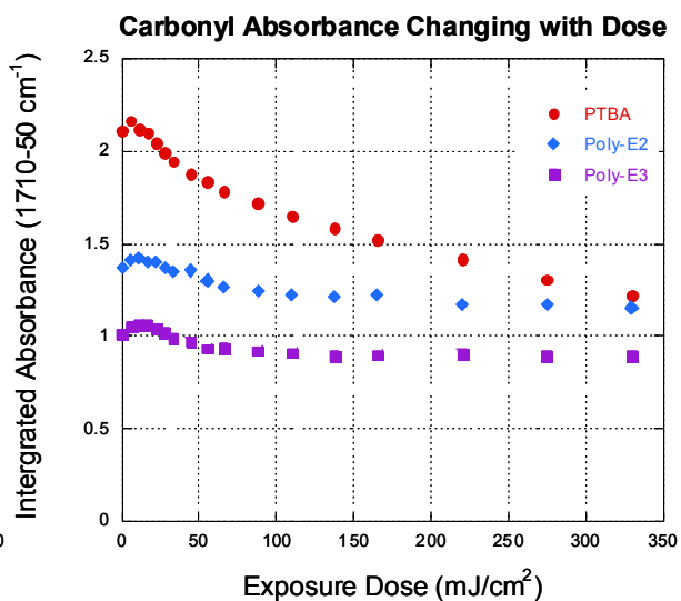
Figure 9. Integrated absorbance of the carbonyl peak of poly(t-butyl acrylate) and two ESCAP copolymers with EUV exposure dose.
