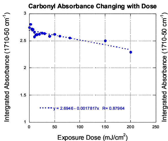
Figure 8. Integrated absorbance of the carbonyl peak of poly(methyl methacrylate) with EUV exposure dose and linear fit of absorbance v. dose.
