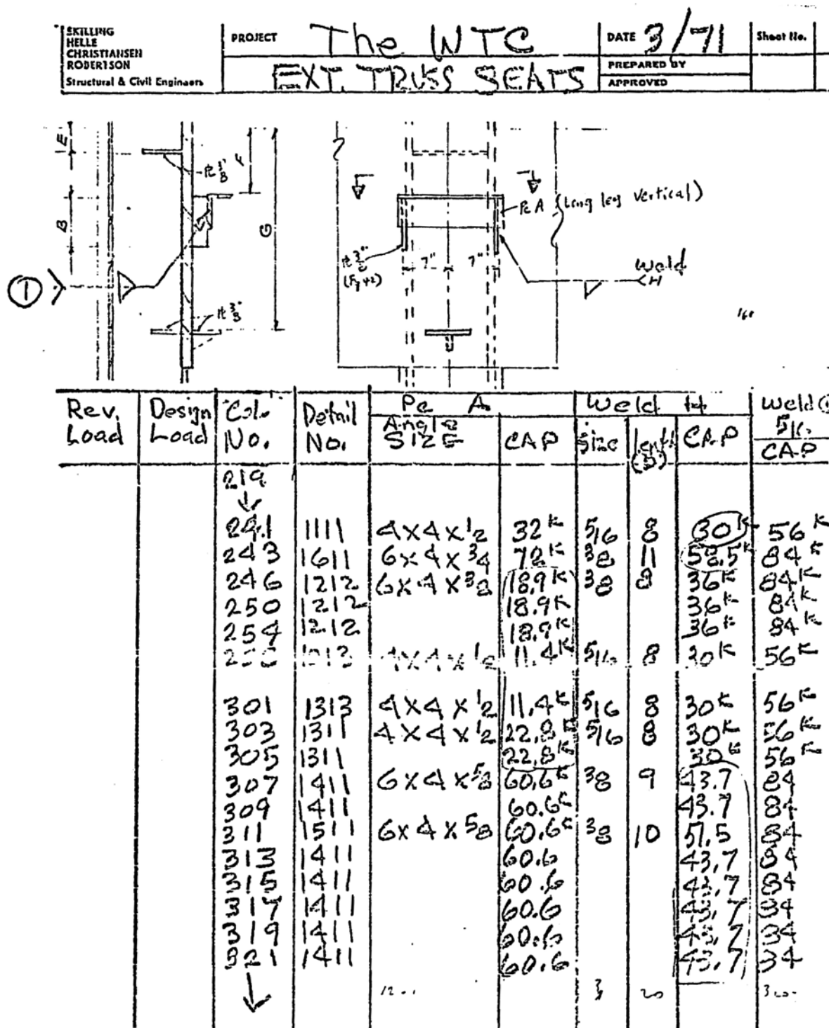
Figure 2-18. Tabulation of component capacities of floor truss connections in WTC 1 and WTC 2 (continued).
