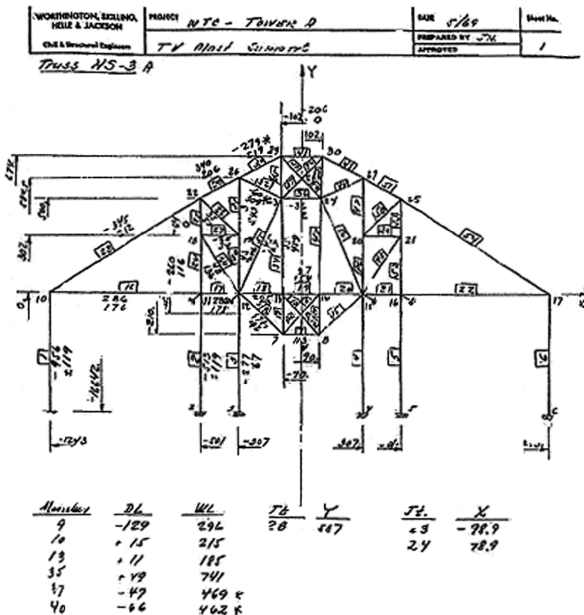
Figure 2-27. Design method for hat trusses in WTC 1 and WTC 2.
