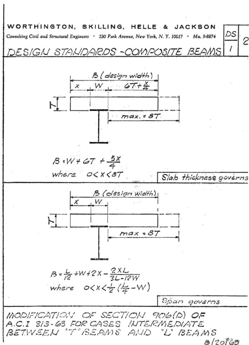
Figure 2–19. Design standard for composite sections in WTC 1 and WTC 2.
