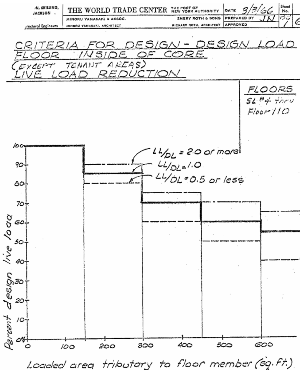
Figure 2-10. Design criteria for WTC 1 and WTC 2: floors inside of core, except for tenant areas – live load reduction.
