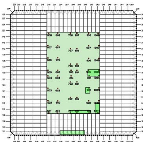
(a) Floor 79
