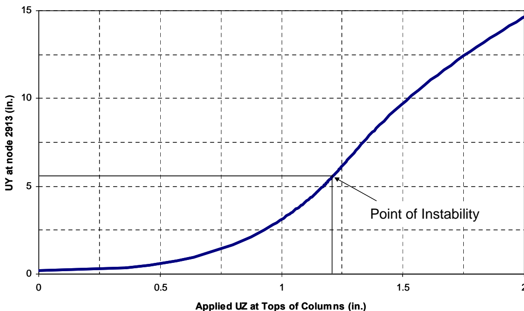
Figure 6-39. Transverse deflection during pushdown after application of temperature DBARE with three unbraced floors.
