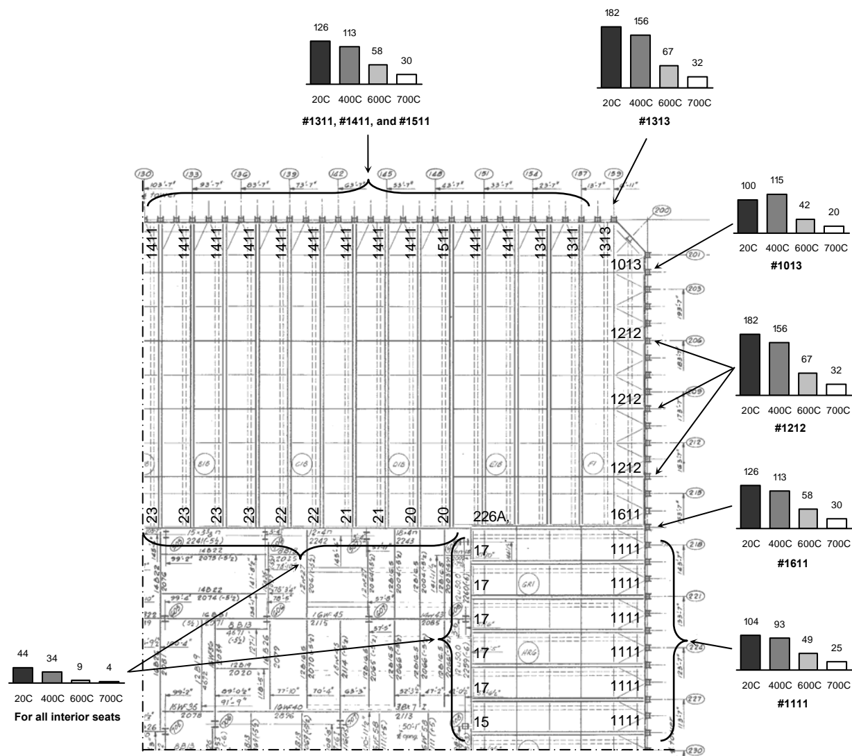
Figure 5–8. Truss seat capacity for horizontal tensile force.
