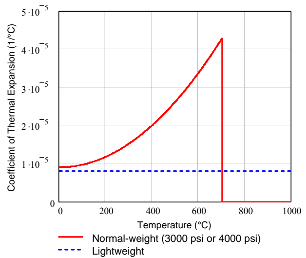
(b) Instantaneous coefficient of thermal expansion
