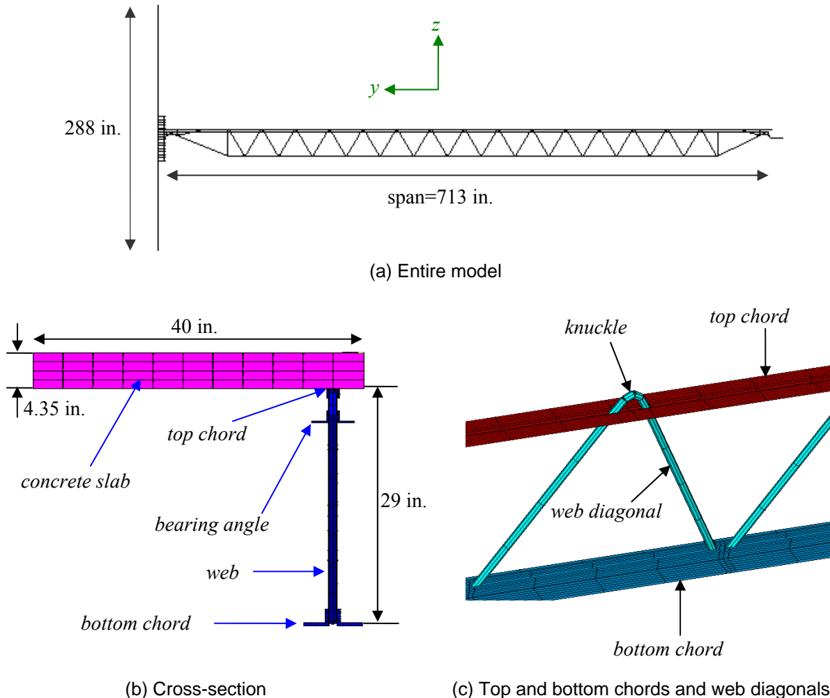
Figure 5-25. Truss model.
