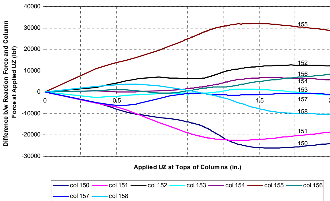
Figure 6-38. Difference between the additional individual column reaction forces at base and the vertical force applied at the top of each column during pushdown after application of temperature DBARE with three unbraced floors.
