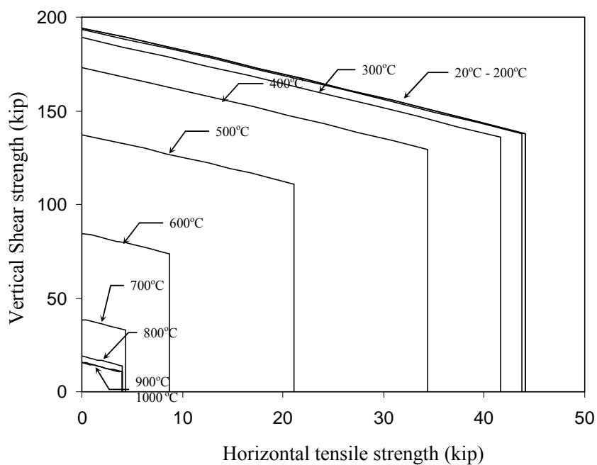
Figure 5–9. Capacity of interior truss seat against vertical and horizontal force (Detail 22).
