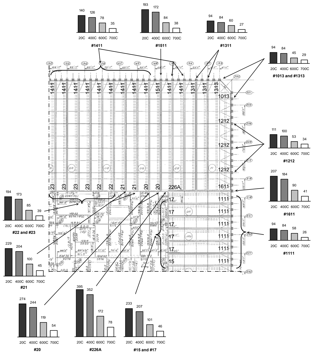
Figure 5-7. Truss seat capacity for vertical force
