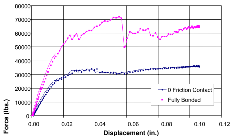
Figure 5–21. Shear force versus displacement from finite element model for longitudinal shear of two knuckles (4,100 psi concrete).
