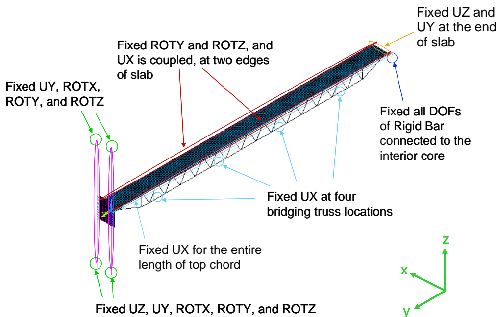
Figure 5–26. Boundary conditions.
