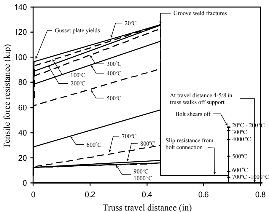
Figure 5–6. Capacity of exterior truss seat for tensile force (Detail 1411).
