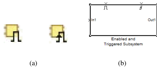
Fig. 12: (a) Enabled and Triggered symbols for systems in SystemBuild; (b) Triggered and Enabled subsystem in Simulink.
