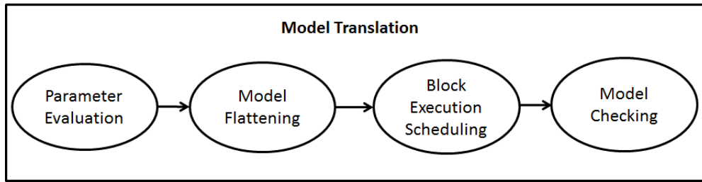
Fig. 14: Model translation
