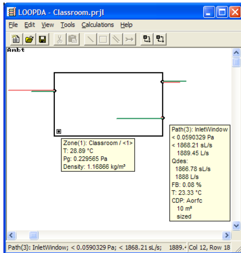
Figure 7 - SketchPad display of analysis calculation (ContamX simulation) results
