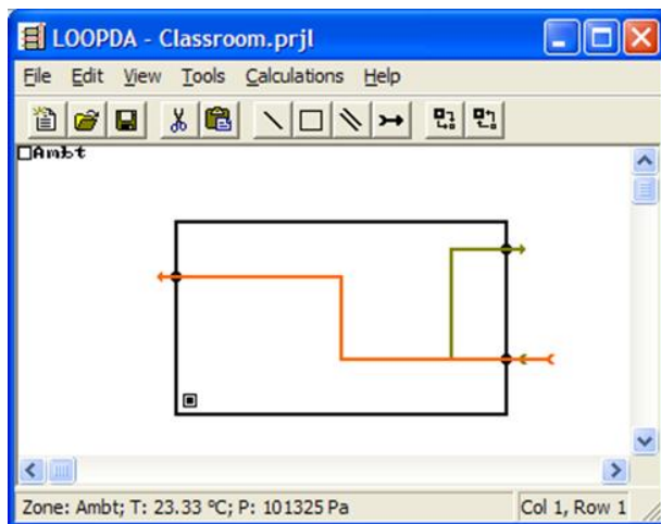
Figure 2 - SketchPad showing zone, paths and loops
