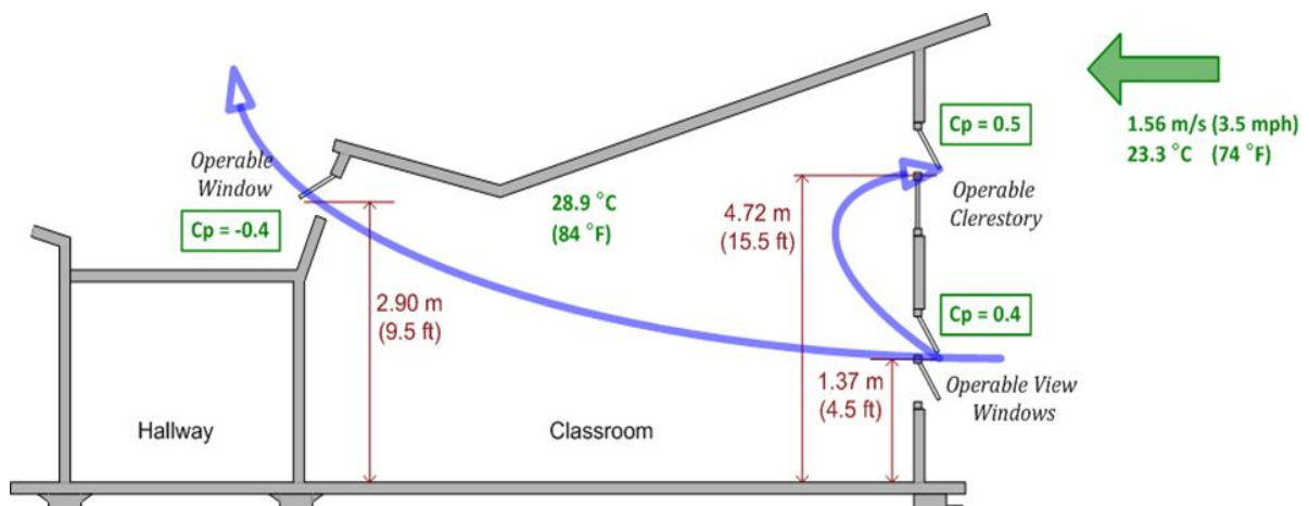
Figure 1 - Conceptualization of Classroom Natural Ventilation Design
