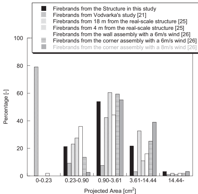
Fig. 13. Comparison of size distributions with Vodvarka [21].
