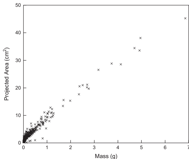
Fig. 10. Size and mass distribution of firebrands collected in this study.
