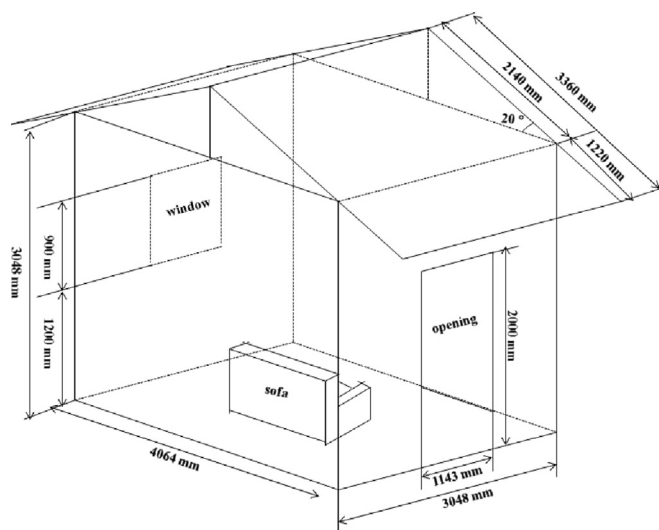
Fig. 1. Schematic of the structure.
