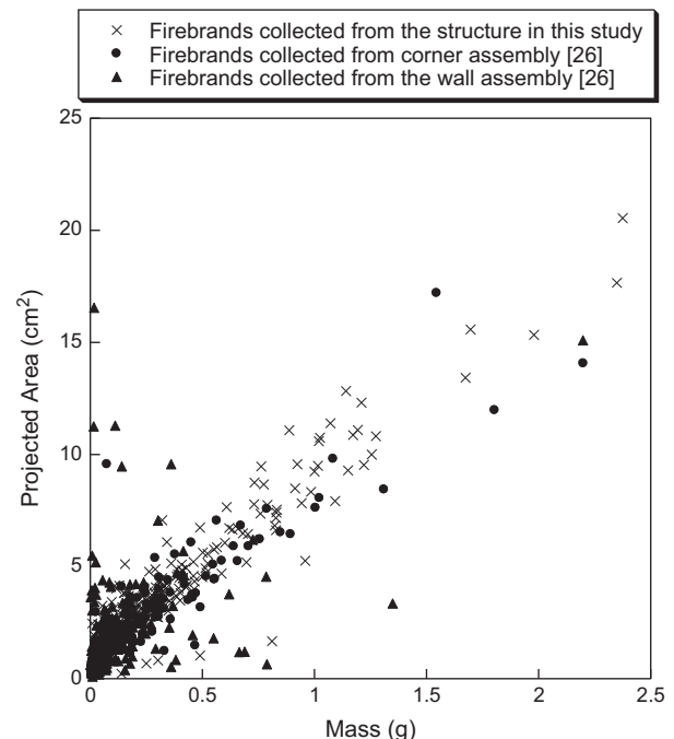
Fig. 12. Comparison of size and mass distribution with components test under the similar laboratory condition [26].
