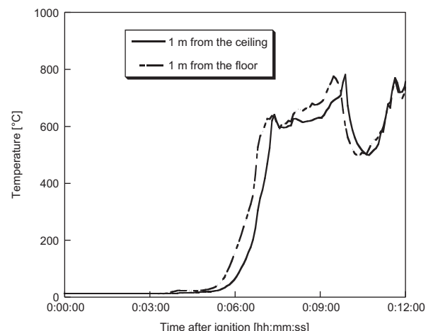
Fig. 9. Temperature profile measured inside the structure.
