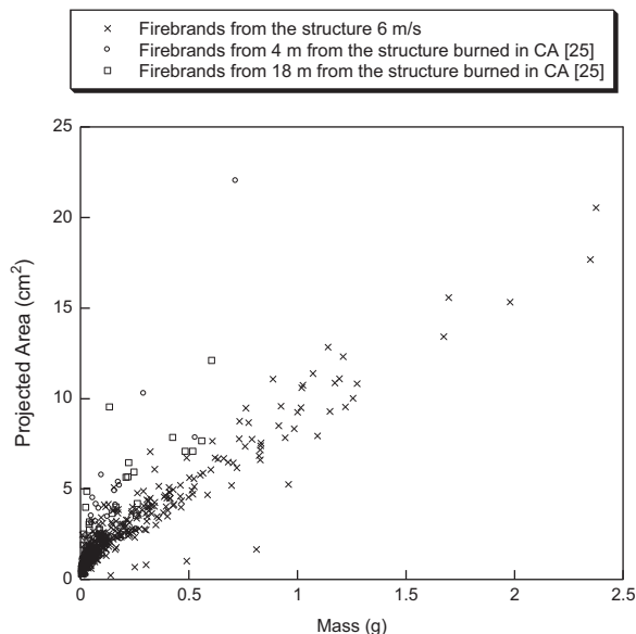
Fig. 11. Comparison of size and mass distribution with full-scale structure burn in Dixon, CA [25].
