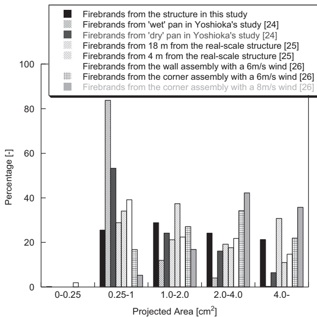
Fig. 14. Comparison of size distributions with Yoshioka et al. [24].
