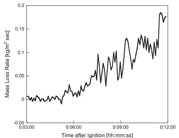
Fig. 6. Temporal profile of mass loss rate per unit area.
