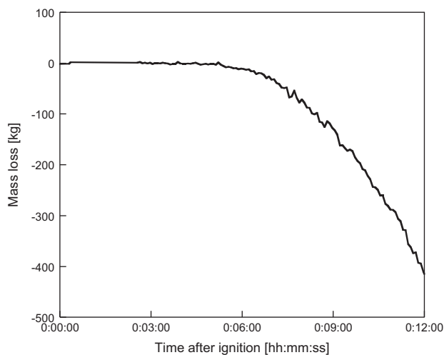
Fig. 5. Temporal profile of mass loss.
