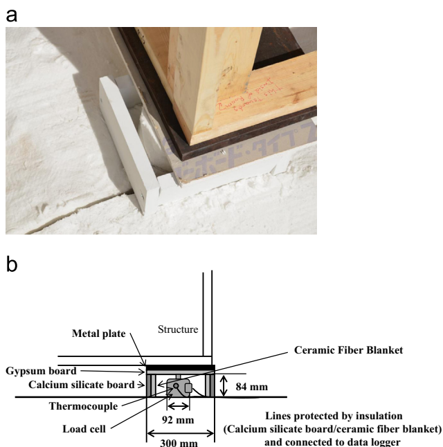
Fig. 7. Images of load cell protection. (a) Picture of load cell protection, (b) schematic of load cell protection.
