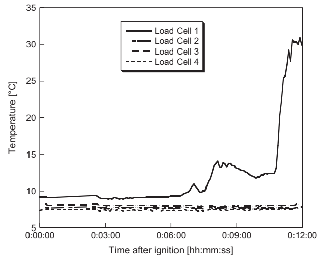
Fig. 8. Temperature profile measured at load cells.
