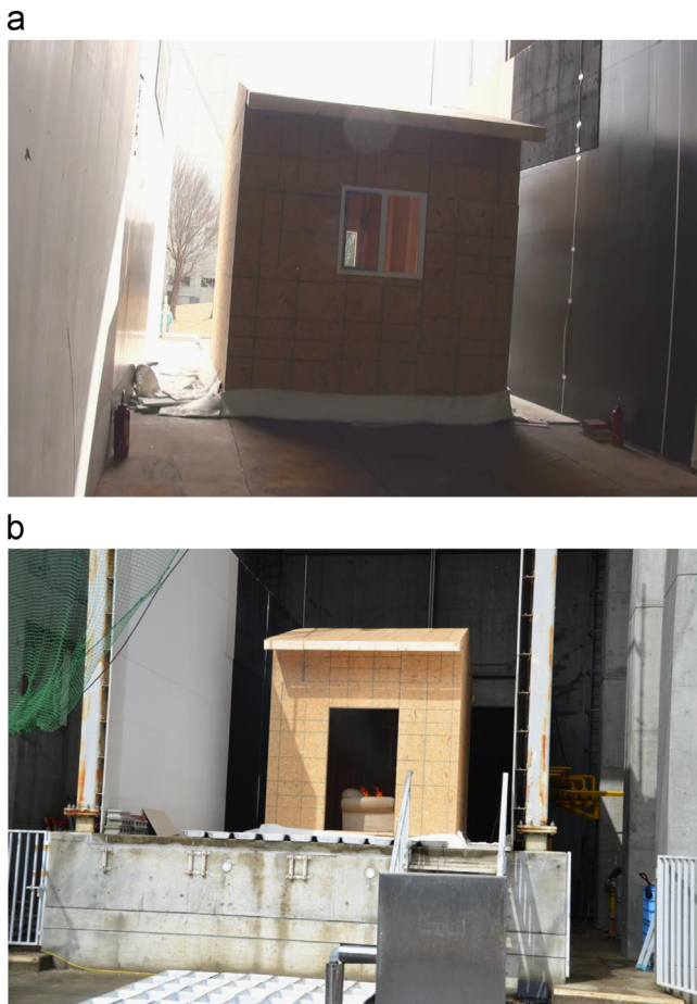
Fig. 2. Pictures of the structure at the onset of the experiment. (a) From inside wind tunnel, (b) from outside wind tunnel.
