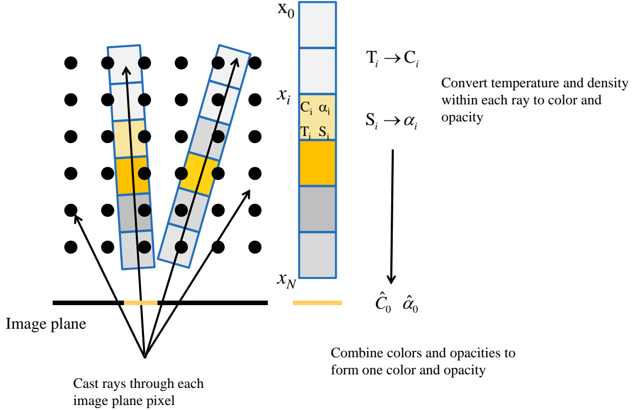
Figure 4.10: Opacity and color is computed for each pixel on an image plane by solving a line integral representation of a simplified form of the radiation transport equation. Rays are cast through the image plane into the 3D data set converting temperatures to color and soot densities to opacity. The line integral is computed for each pixel where the ray intersects the data set.
