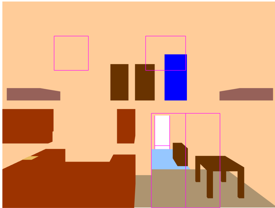
flat shading
