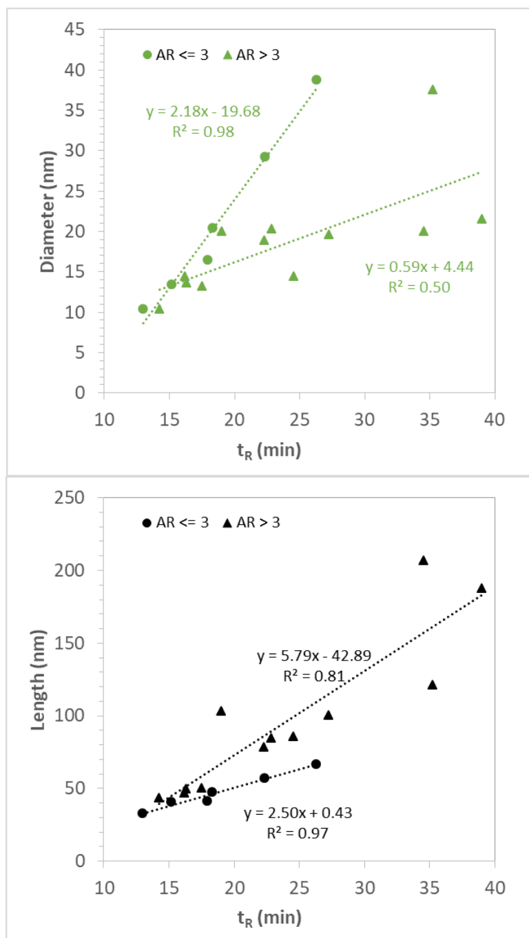
Figure S6: Diameter and length as a function of retention time for aspect ratio \leq 3 or > 3 .
