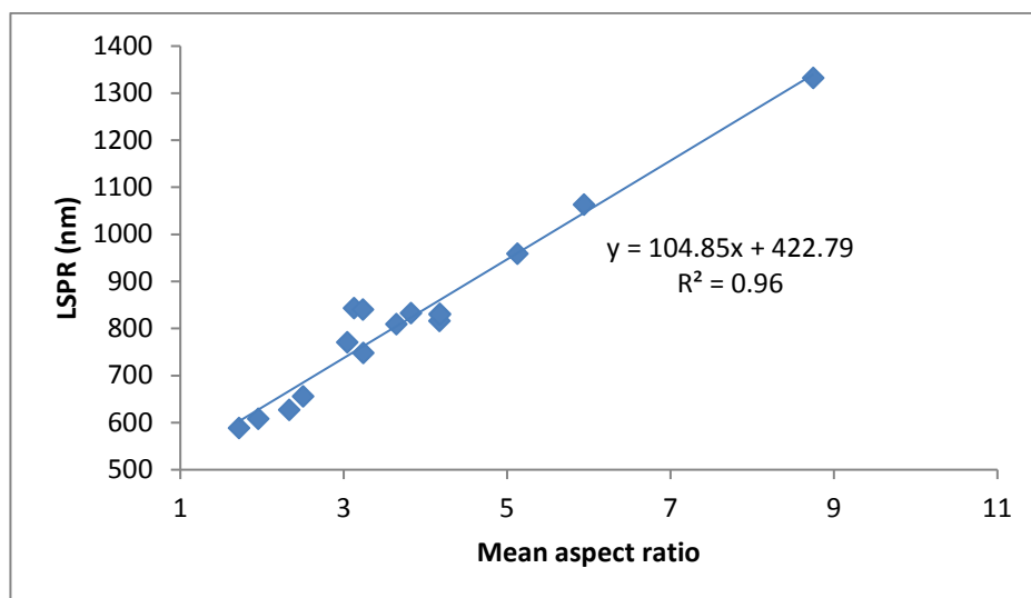
Figure S2: relationship between the measured LSPR and the mean calculated AuNR AR based on TEM analysis.
