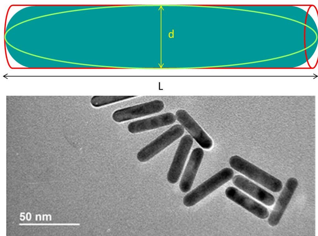
Figure S3: Structure of a gold nanoparticle (blue filled) compared to cylinder (red) and prolate ellipsoid (green) shapes.
